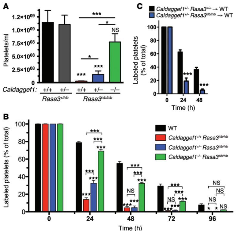
Figure 3. Platelet number and life span in Rasa3 h/b/h/b mice are normalized by reducing CalDAG-GEFI expression. (A and B) Deletion of CalDAG-GEFI restores the peripheral platelet count and platelet life span in Rasa3 h/b/h/b mice. (A) Whole blood samples were obtained from controls and Caldaggef1 +/- Rasa3 h/b/h/b , Caldaggef1 +/- Rasa3 h/b/h/b , and Caldaggef1 -/- Rasa3 h/b/h/b mice, and platelet counts per ml blood were determined ( n = 6). (B) Whole blood samples were obtained from WT, Caldaggef1 +/- Rasa3 h/b/h/b , Caldaggef1 +/- Rasa3 h/b/h/b , and Caldaggef1 -/- Rasa3 h/b/h/b mice at the indicated time points after injection of anti-GPIX Alexa Fluor 488, and the fraction of labeled to unlabeled platelets was determined ( n = 6). * P < 0.05, *** P < 0.0001, 2-way ANOVA with Bonferroni post-test. (C) Reduced platelet half-life in Rasa3 h/b/h/b mice is caused by a defect that is intrinsic to platelets. The bar graph shows the survival of Caldaggef1 +/- Rasa3 +/- or Caldaggef1 +/- Rasa3 h/b/h/b platelets after transfusion into WT recipient mice ( n = 6). *** P < 0.0001, 2-tailed Student's t test.
